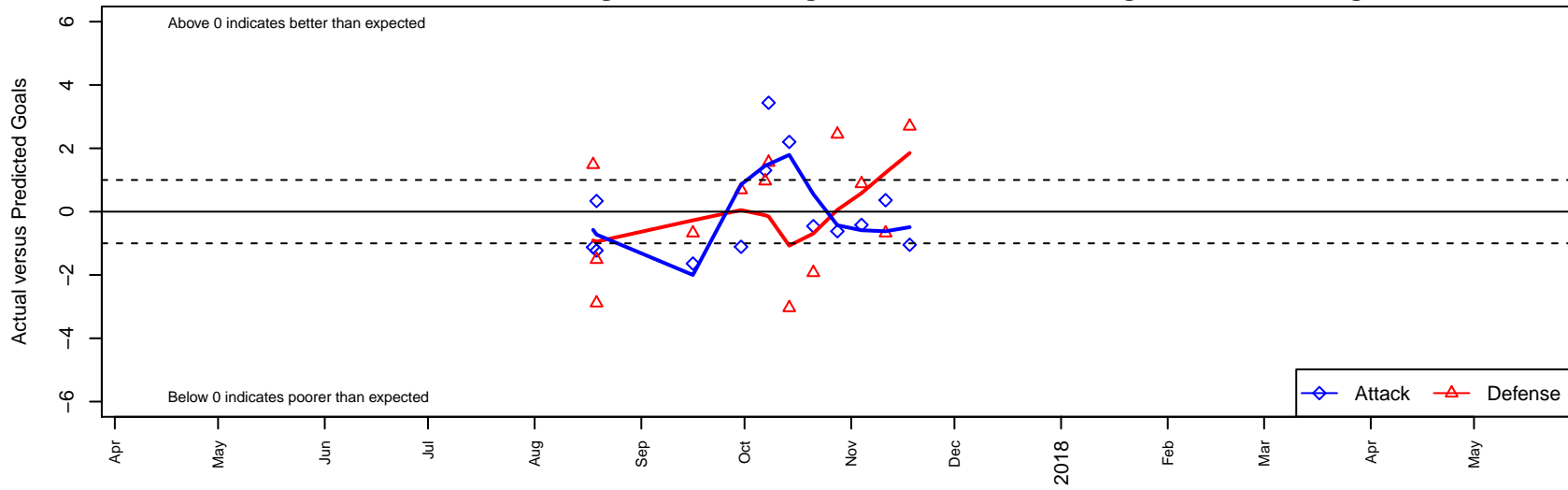
Central WA SA White B04 Dots are actual minus expected GF (blue circles) and GA (red triangles). Blue line is smoothed change in attack strength. Red is smoothed change in defense strength.
